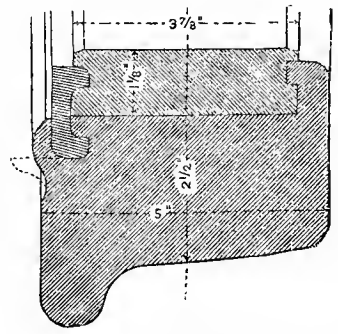
Fig. 5343 DRUMMOND FASTENING.
